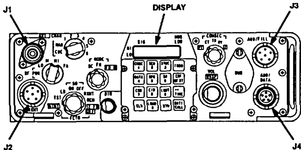
RT-1523C/D (SIP) FRONT PANEL
