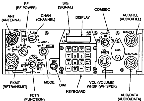
RT-1523/A/B FRONT PANEL
